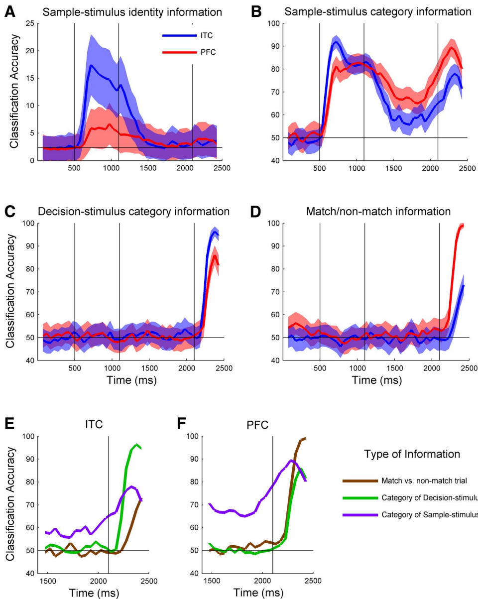
FIG. 2. Basic decoding results for 4 different types of information. A–D: blue lines indicates results from inferior temporal cortex (ITC) and red lines indicate results from prefrontal cortex (PFC; red, and blue shaded regions indicate one SD over the bootstrap-like trials). The 3 vertical black lines indicate SAMPLE-STIMULUS onset, SAMPLE-STIMULUS offset, and DECISION-STIMULUS onset from left to right respectively. E and F: comparison of SAMPLE-STIMULUS category decoding accuracy (purple), DECISION-STIMULUS category decoding accuracy (green), and whether a trial is a match or nonmatch trial (brown) for ITC (E) and PFC (F).
